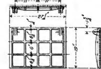
Figs. 665-667. Slide for Ashpan Drop
